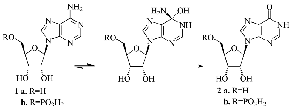
SCHEME 1 ADA- and AMPDA-catalyzed deamination of adenosine ( 1a ) and adenosine 5'-phosphate ( 1b ).
