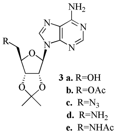
FIGURE 1 Structure of adenosine analogues 3a–e
