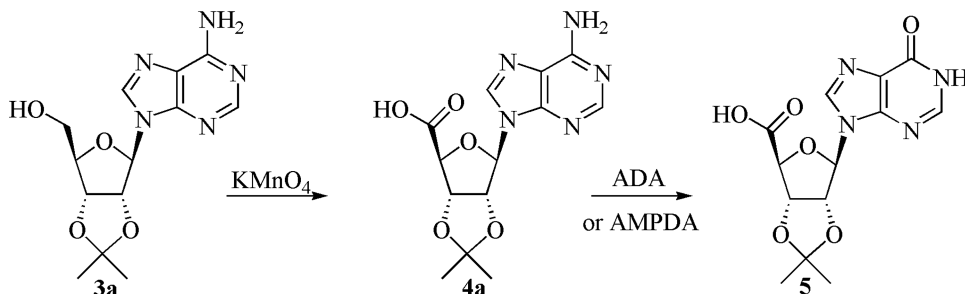
SCHEME 2 Synthesis of 2',3'-isopropylideneadenosine-5'-carboxylic acid ( 4a ) and related enzyme-catalyzed deamination to inosine derivative 5 .
