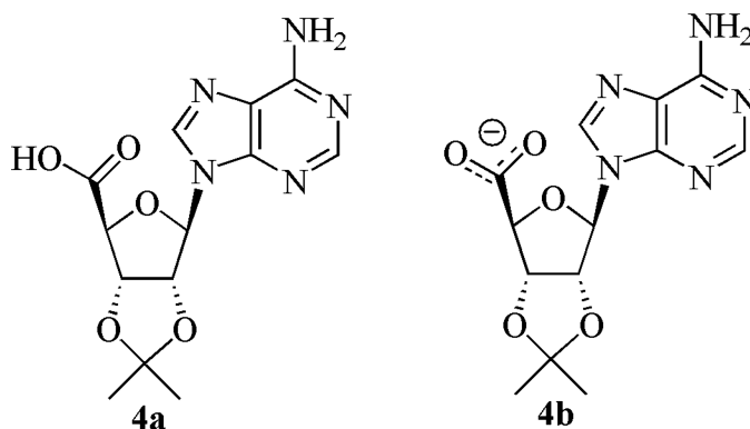
FIGURE 2 Structure 2',3'-isopropylideneadenosine-5'-carboxylic acid in uncharged and charged forms ( 4a and 4b ).
